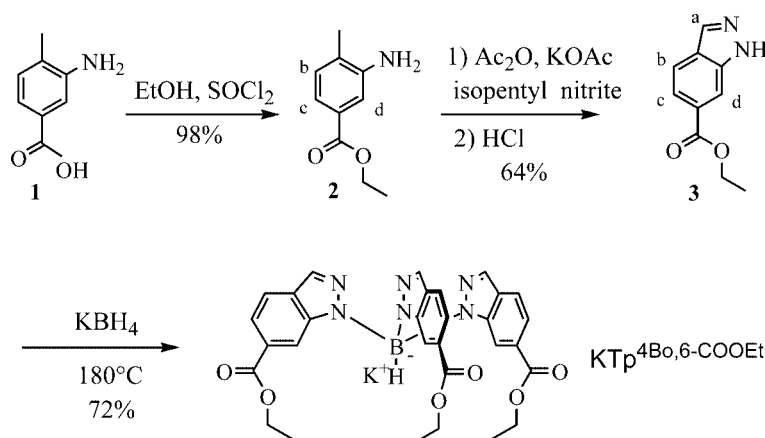
Scheme 1. Synthesis of potassium hydrotris[6-(ethoxycarbonyl)indazol-1-yl]borate.
