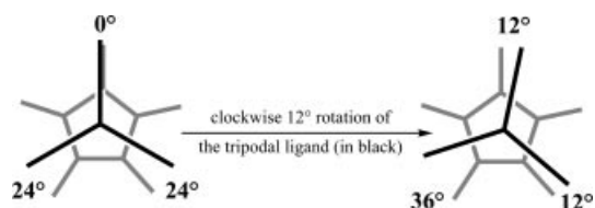
Figure 3. Eclipsed (left) and staggered (right) conformations of a complex containing both C_3 - and C_5 -symmetry ligands. Interconversion occurs upon a 12^\circ rotation. For symmetry reasons, the staggered conformation appears every 24^\circ .
