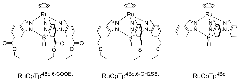
Figure 1. Structure of the triester-functionalized, trithioether-functionalized, and unfunctionalized ruthenium(II) complexes.
