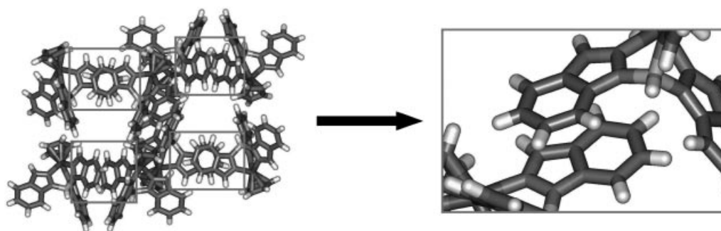
Figure 4. Stabilization in the crystal structure of \text{RuCpTp}^{4\text{Bo}} by \pi -stacking interactions between neighboring indazolyl pairs. Zooming in shows the donor–acceptor interactions between two indazolyl groups positioned in a head-to-tail arrangement with an interplane distance of 3.56 \text{ \AA} .
