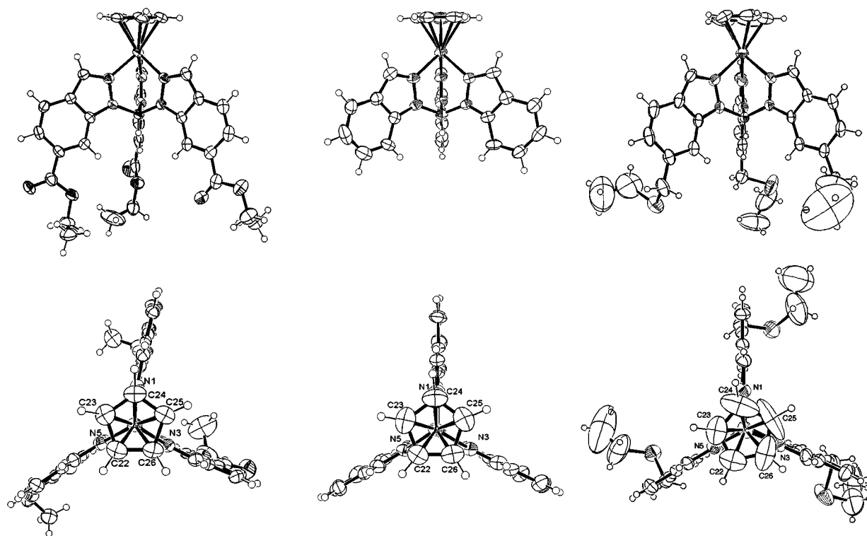
Figure 2. Thermal ellipsoid diagram of (\text{RuCpTp}^{4\text{Bo},6\text{-COOEt}}) (left), (\text{RuCpTp}^{4\text{Bo}}) (center), and (\text{RuCpTp}^{4\text{Bo},6\text{-CH}_2\text{SEt}}) (right), side view (top) and top view (bottom). The ellipsoids are drawn at the 50% probability level and the molecules of cocrystallizing solvent (MeOH) have been removed for clarity.
