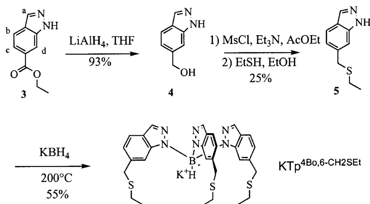
Scheme 2. Synthesis of potassium hydrotris[6-[(ethylsulfanyl)methyl]indazol-1-yl]borate.
